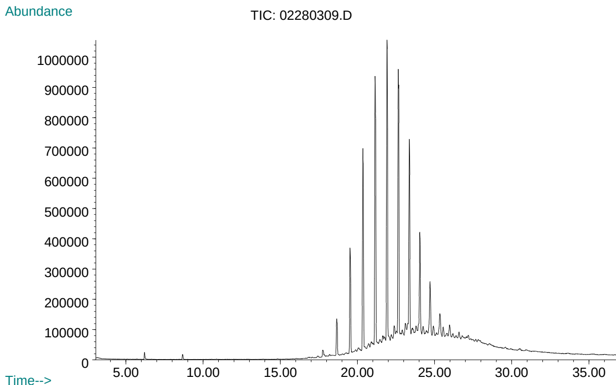
Figure 13. GC/MS (Gas Chromatography/Mass Spectrometry) extractables profile (Total Ion Chromatogram, TIC) of the peroxide-cured elastomer test article, 2-propanol sonication extract.
