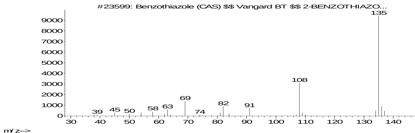
Figure 27. Electron ionization (EI) mass spectrum of extractable peak #5 from Table 3 (top) with best fit mass spectral library match (bottom) or benzothiazole.
