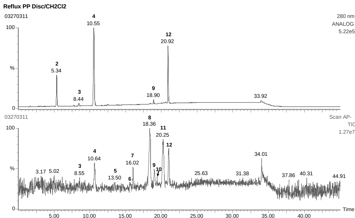
3025 Figure 21. HPLC-UV chromatogram and negative ion Total Ion Chromatogram 3026 polypropylene disc, 4-hour methylene chloride reflux extract.
