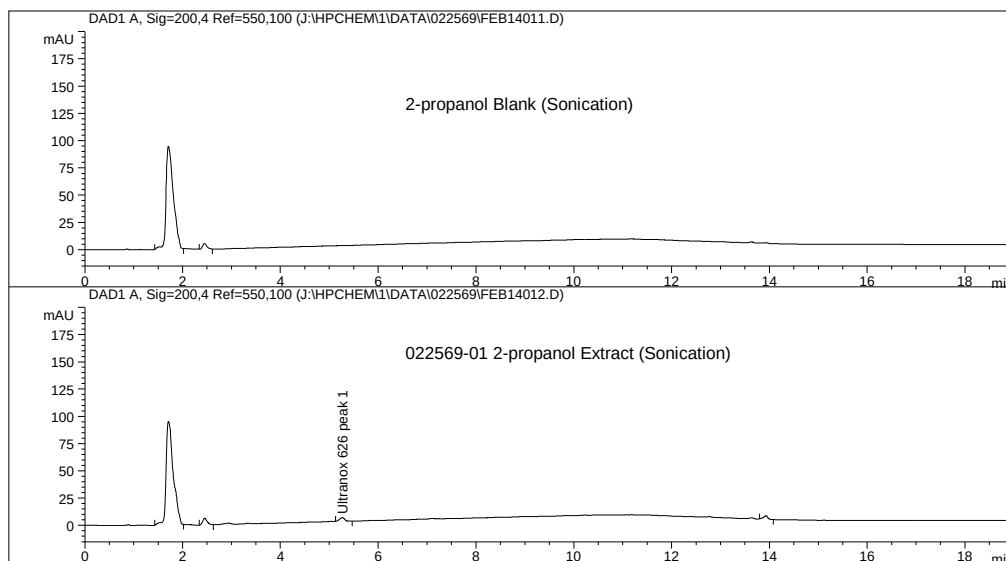
Figure 15. HPLC/DAD (High Performance Liquid Chromatography/Diode Array Detection) extractables profile (UV@200 nm) of a polypropylene test article 2-propanol sonication extract. The labeled peak at approximately 5.5 minutes is di- tert -butyl phenol from Ultranox 626.
