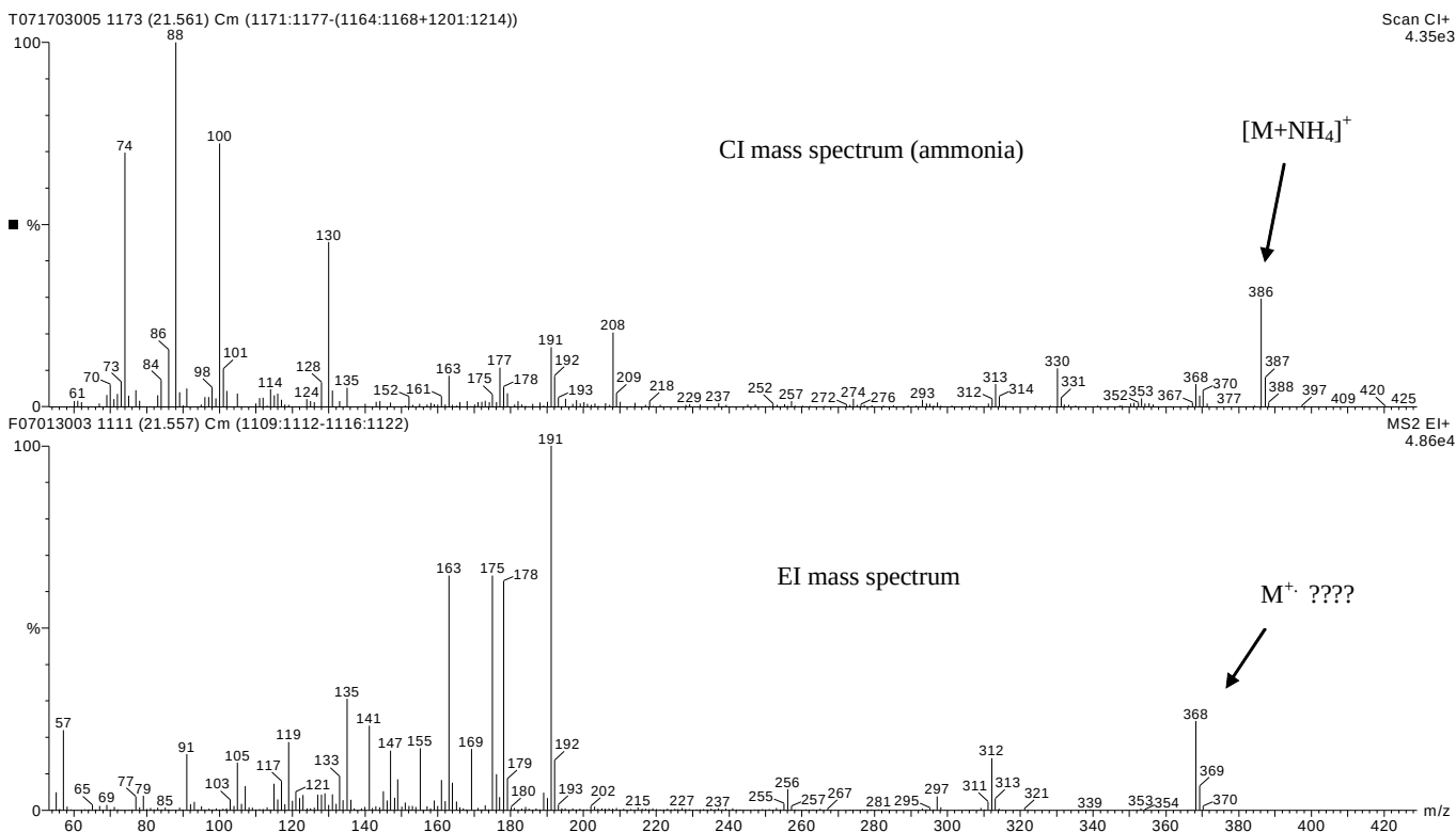
Figure 26. Ammonia chemical ionization (CI) mass spectrum (top) and electron ionization (EI) mass spectrum (bottom) of 2,2'-methylene-bis-(-6- tert -butyl)-4-ethylphenol (peak #35 in Table 3). Note that the [M+NH_4]^+ at m/z 386 in the CI spectrum confirms m/z 368 in the EI spectrum as the molecular ion ( M^+ ), and therefore represents the molecular weight of the extractable.
