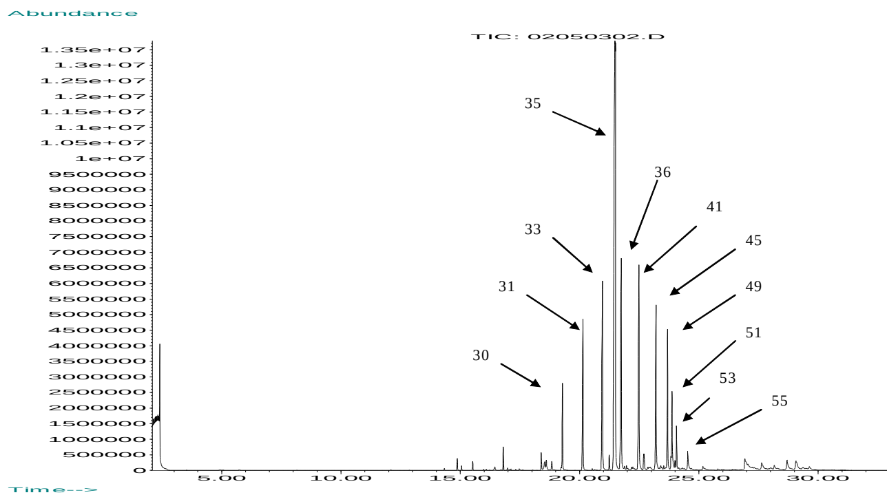
Figure 25. GC/MS (Gas Chromatography/Mass Spectrometry) extractables profile (Total Ion Chromatogram, TIC) of the sulfur cured elastomer test article, methylene chloride Soxhlet extract.
