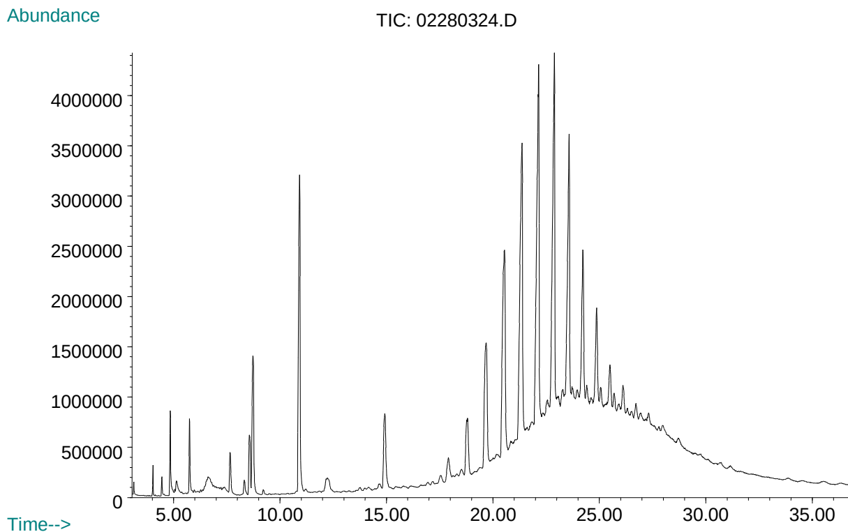
Figure 12. GC/MS (Gas Chromatography/Mass Spectrometry) extractables profile (Total Ion Chromatogram, TIC) of the peroxide-cured elastomer test article, 2-propanol reflux extract.
