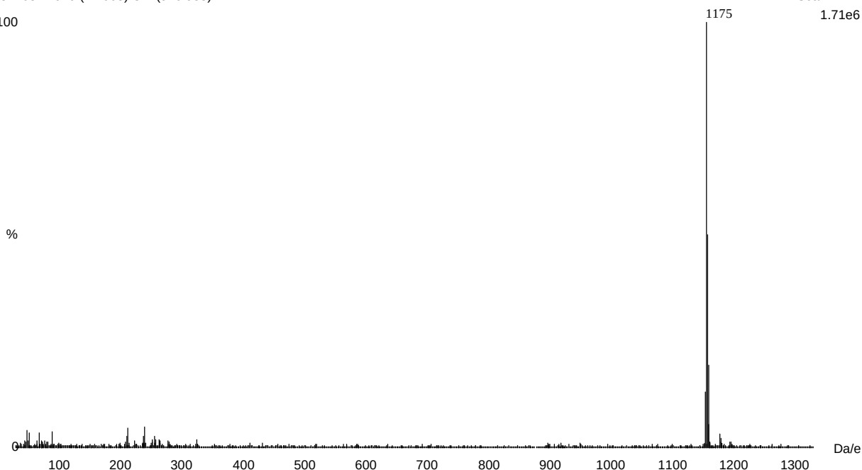
Figure 23. Negative ion APCI mass spectrum of Irganox 1010. Note the [M-H]^- at m/z 1175.
