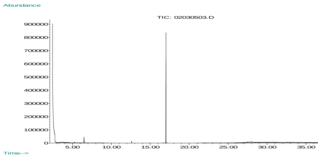
Figure 32. Total Ion Chromatogram from the GC/MS analysis of authentic tetramethylthiuram monosulfide.
