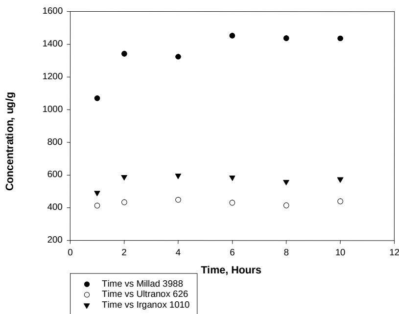
Figure 31. Model extraction optimization experiment (2-propanol reflux extraction) performed during Controlled Extraction Studies on the polypropylene test article.
