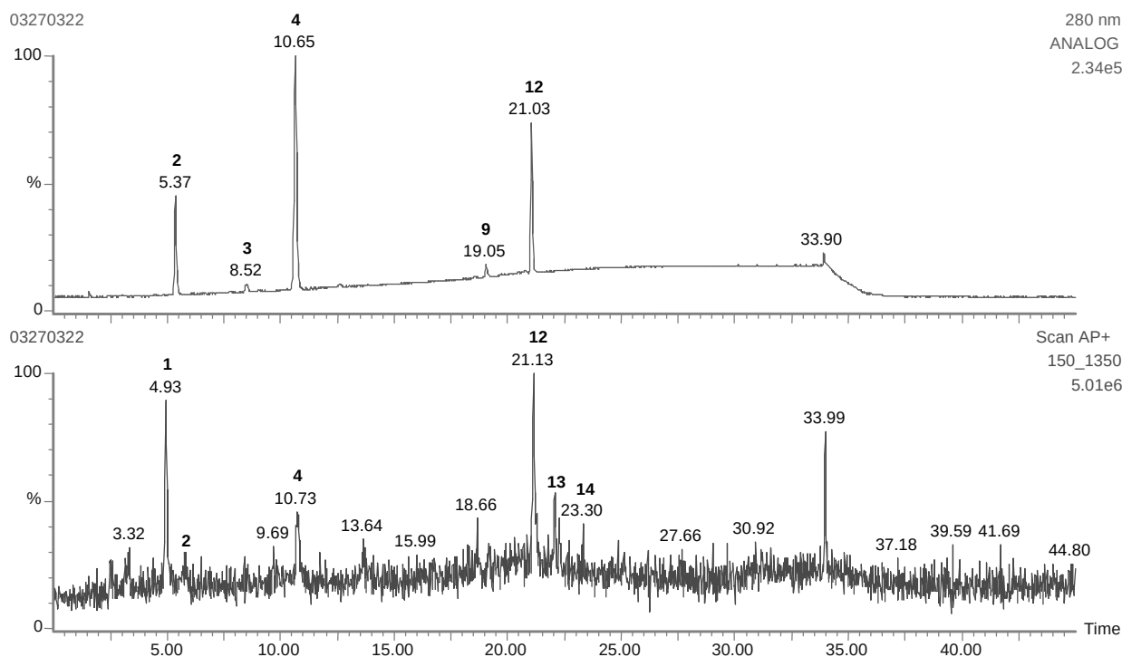
Figure 24. HPLC-UV chromatogram and positive ion Total Ion Chromatogram polypropylene disc, 4-hour methylene chloride reflux extract.
