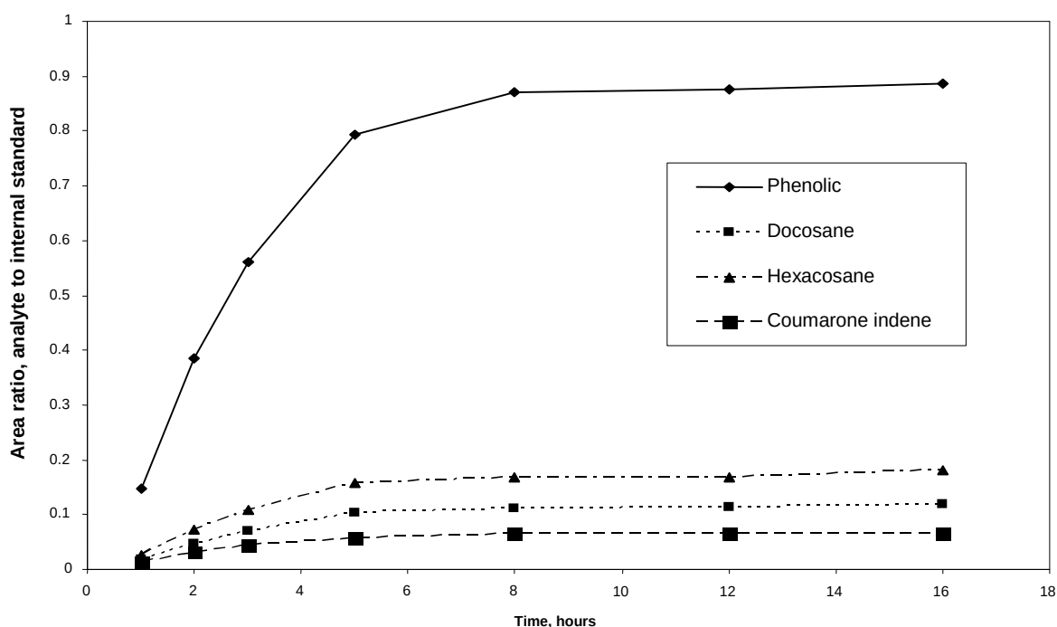
Figure 30. Model extraction optimization experiment (methylene chloride Soxhlet extraction) performed during Controlled Extraction Studies on the sulfur-cured elastomer test article. “Phenolic” = 2,2′-methylene-bis(6- tert -butyl-4-ethylphenol). “Coumarone indene” = coumarone indene resin identified as a trimer of two indenenes with one \alpha -methylstyrene.
