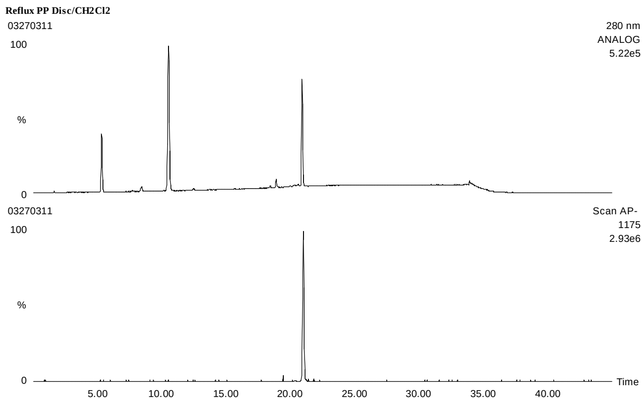
Figure 22. HPLC-UV chromatogram and m/z 1175 extracted ion current profile polypropylene disc, 4-hour methylene chloride reflux extract.
