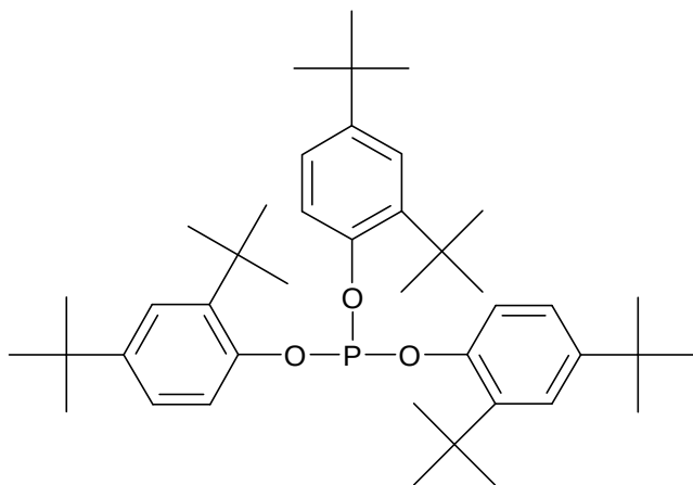
(I) Irgafos 168
