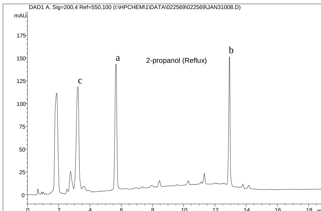
Figure 2. HPLC/DAD (High Performance Liquid Chromatography/Diode Array Detection) extractables profile (UV@200 nm) of a polypropylene test article 2-propanol reflux extract. a = di- tert -butylphenol from Ultrinox 626; b = Tetrakis [methylene (3,5-di- tert -butyl-4-hydroxyhydrocinnamate)] methane; c = 3,4-dimethyl dibenzylidene sorbitol. The peak at approximately 2 minutes represents 2-propanol.
