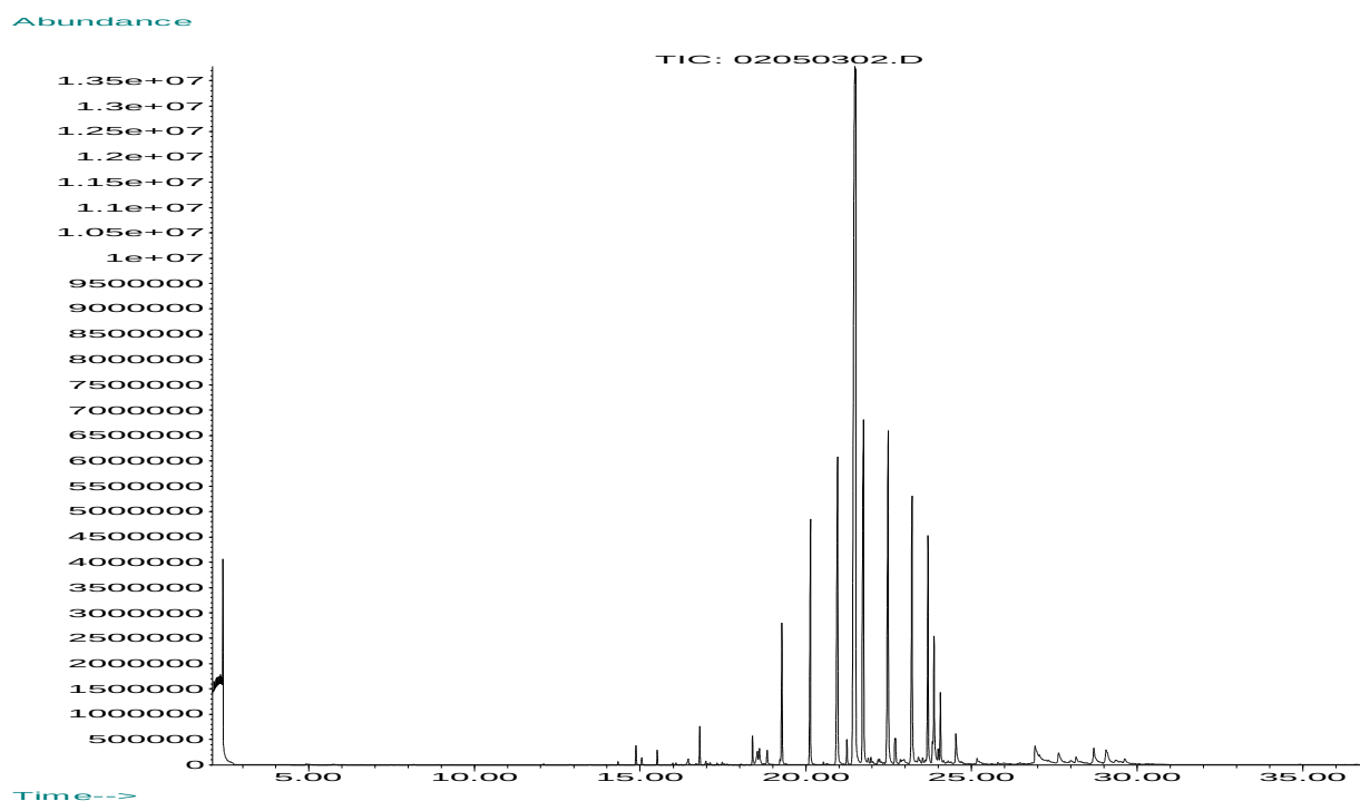
3643 Figure 1. GC/MS (Gas Chromatography/Mass Spectrometry) extractables profile (Total 3644 Ion Chromatogram, TIC) of the sulfur-cured elastomer test article, 24 hour 3645 methylene chloride Soxhlet extraction. 3646 3647
