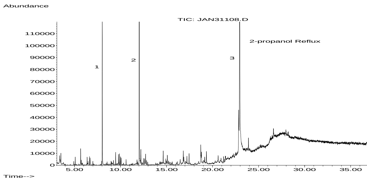
Figure 20. GC/MS analysis of extracts from reflux of polypropylene in 2-propanol. Peak 1 = 2,6-di-methyl benzaldehyde. Peak 2 = 2,4-di- tert -butylphenol. Peak 3 = glycerol monostearate.
