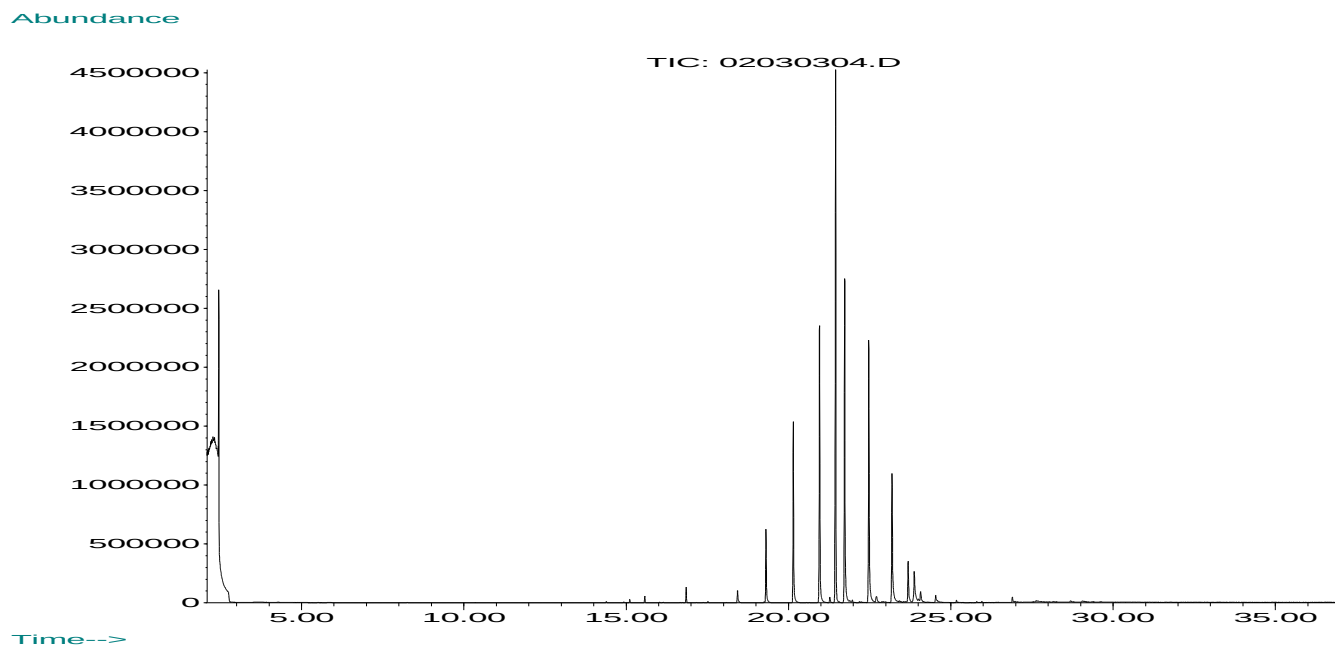
Figure 9. GC/MS (Gas Chromatography/Mass Spectrometry) extractables profile (Total Ion Chromatogram, TIC) of the sulfur-cured elastomer test article, 2-propanol sonication extract. Sample reconstituted in methylene chloride prior to GC/MS analysis.
