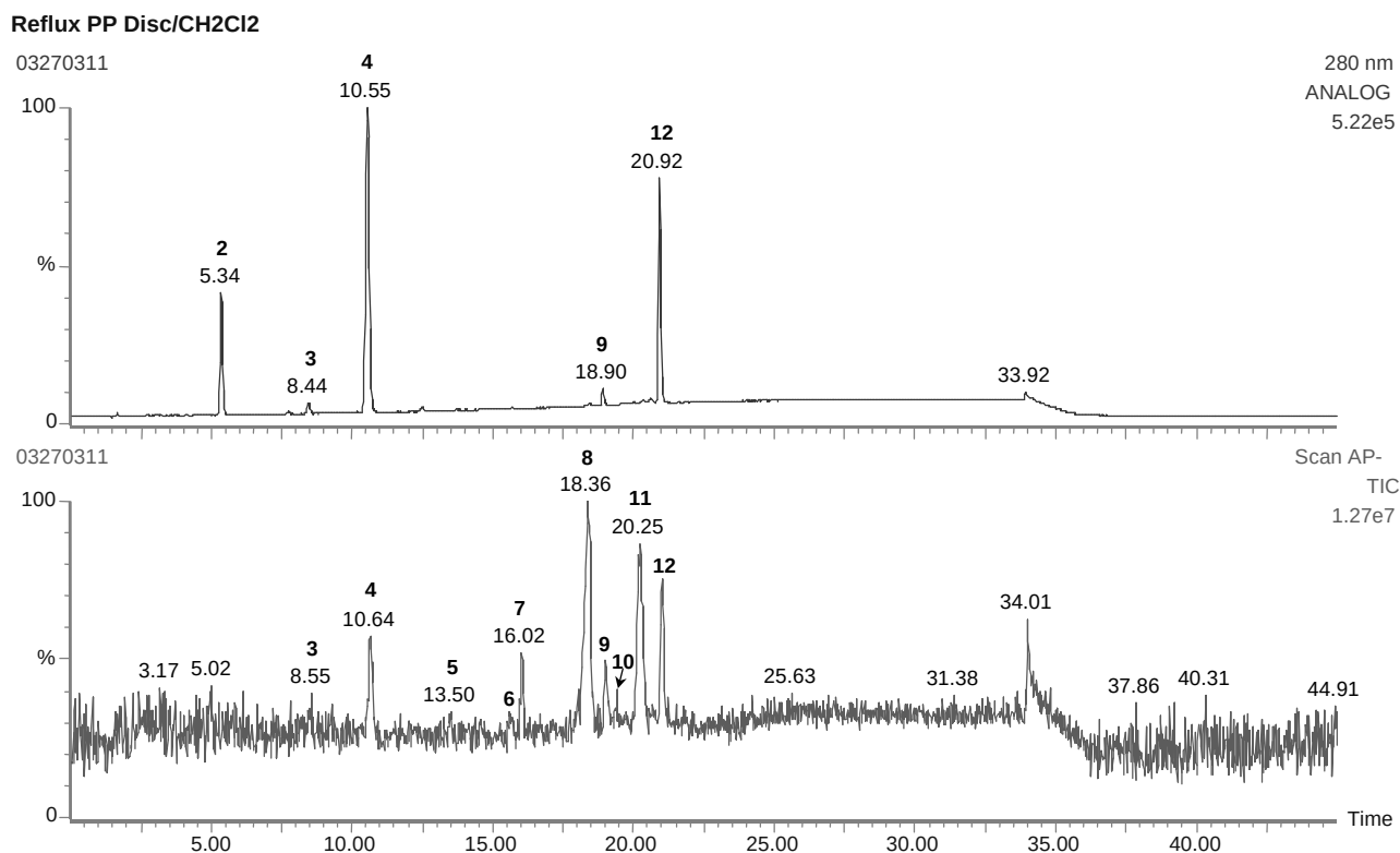
Figure 19. In-line HPLC/UV (@280 nm) and negative ion Total Ion Chromatogram (TIC) extractables profiles of a polypropylene test article methylene chloride reflux extract (see Table 1 for peak identifications). Note that the sample was injected onto the HPLC in a mobile phase mixture.
